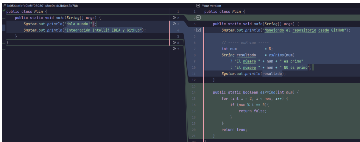
Figura 5: Interfaz « Diff »
