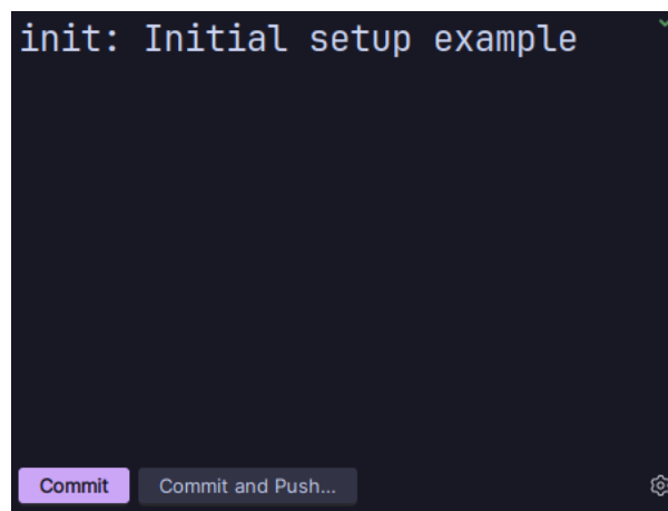
Figura 23: Commit message
